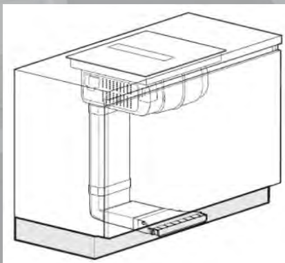
Plinth-Out installation
