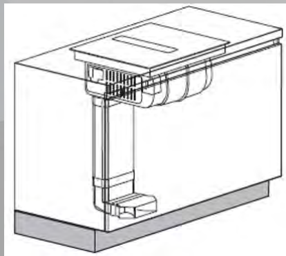
Plinth-In installation
